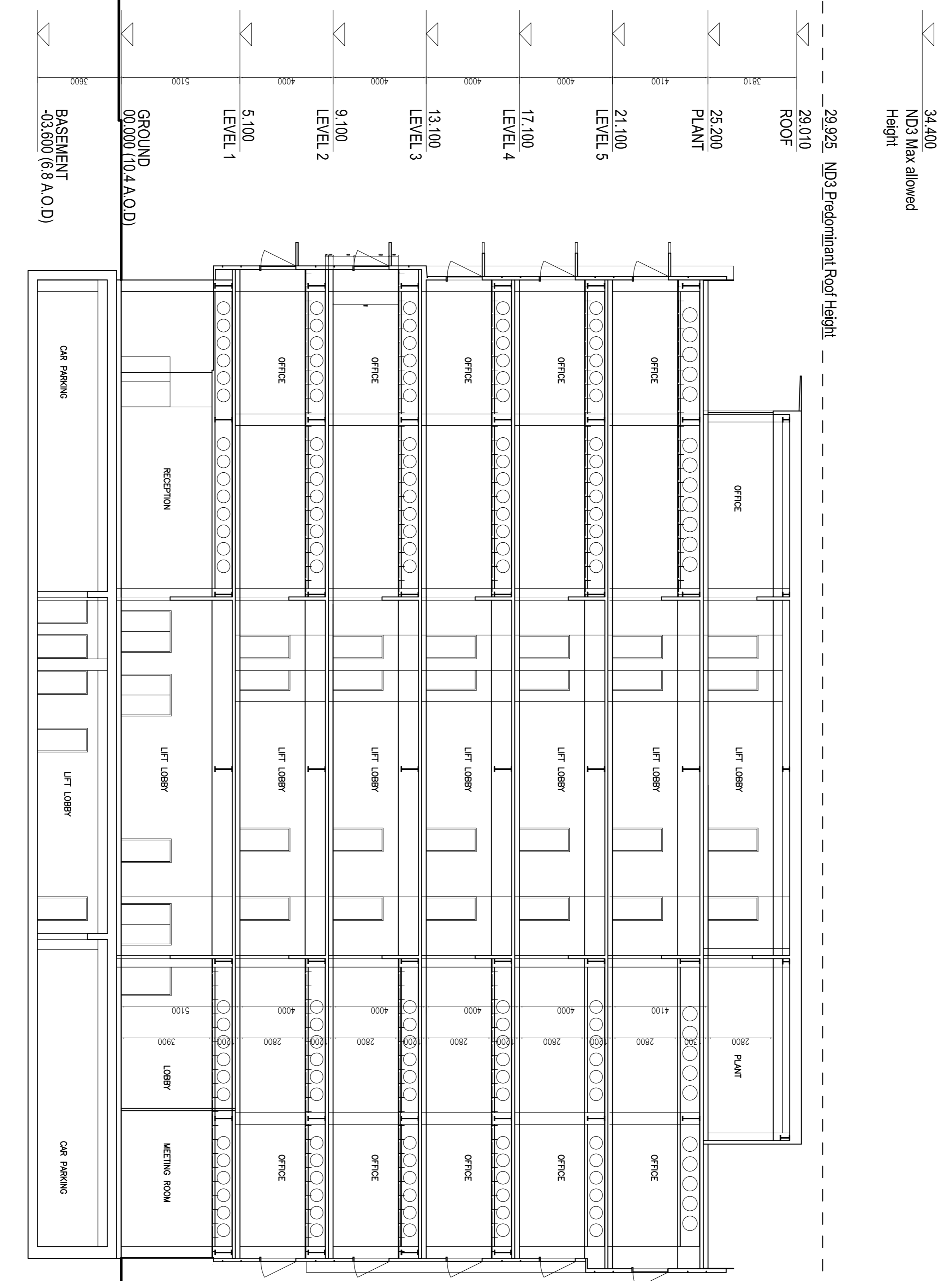
SECTION BB
